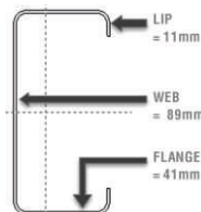
DETAIL SECTION PROFILE
