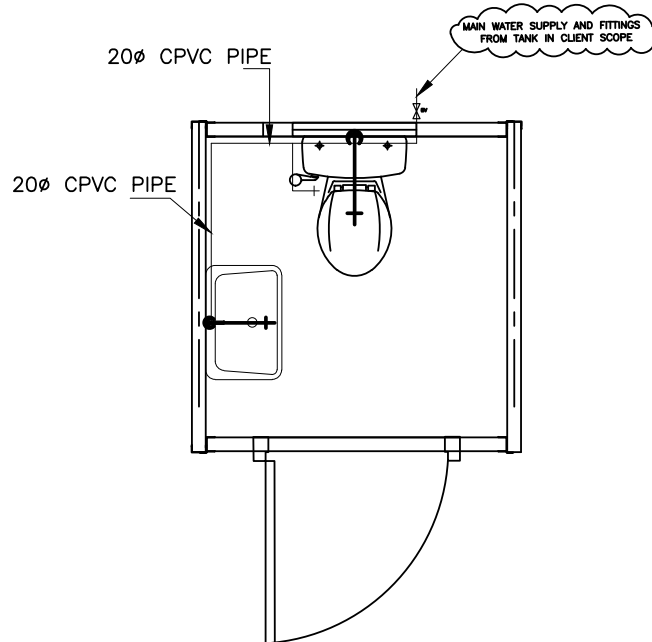
WATER SUPPLY PLAN
