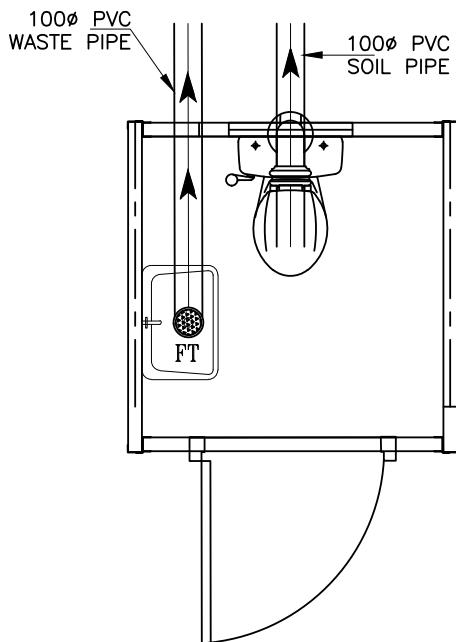
SANITARY PLAN
